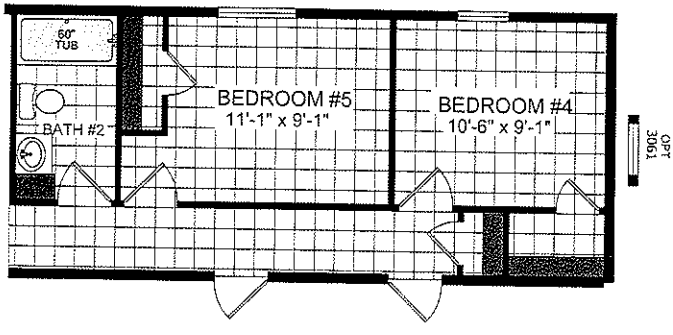
OPT. BEDROOM #5
